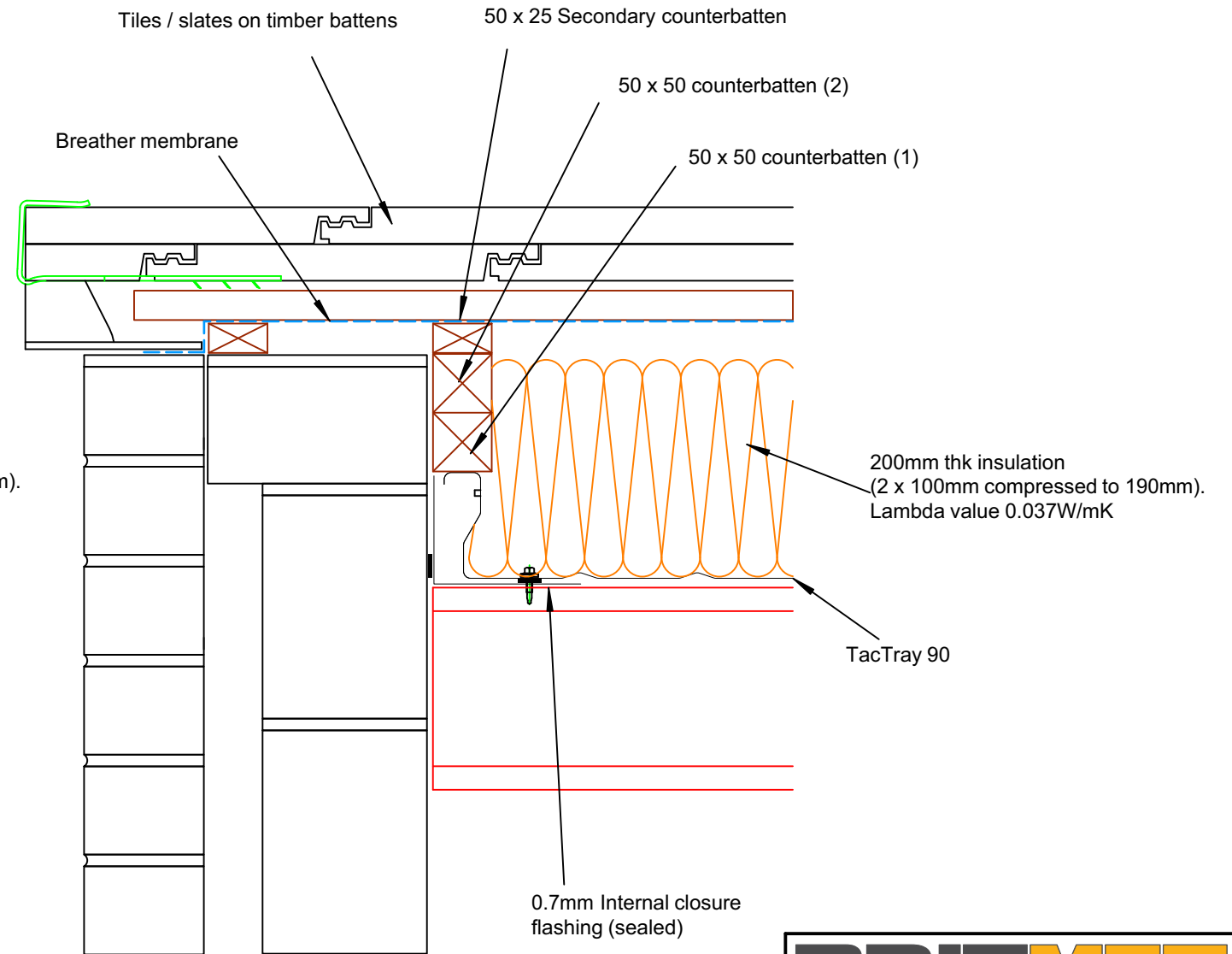
VERGE DETAIL (LEVEL WITH BOUNDARY WALL)
