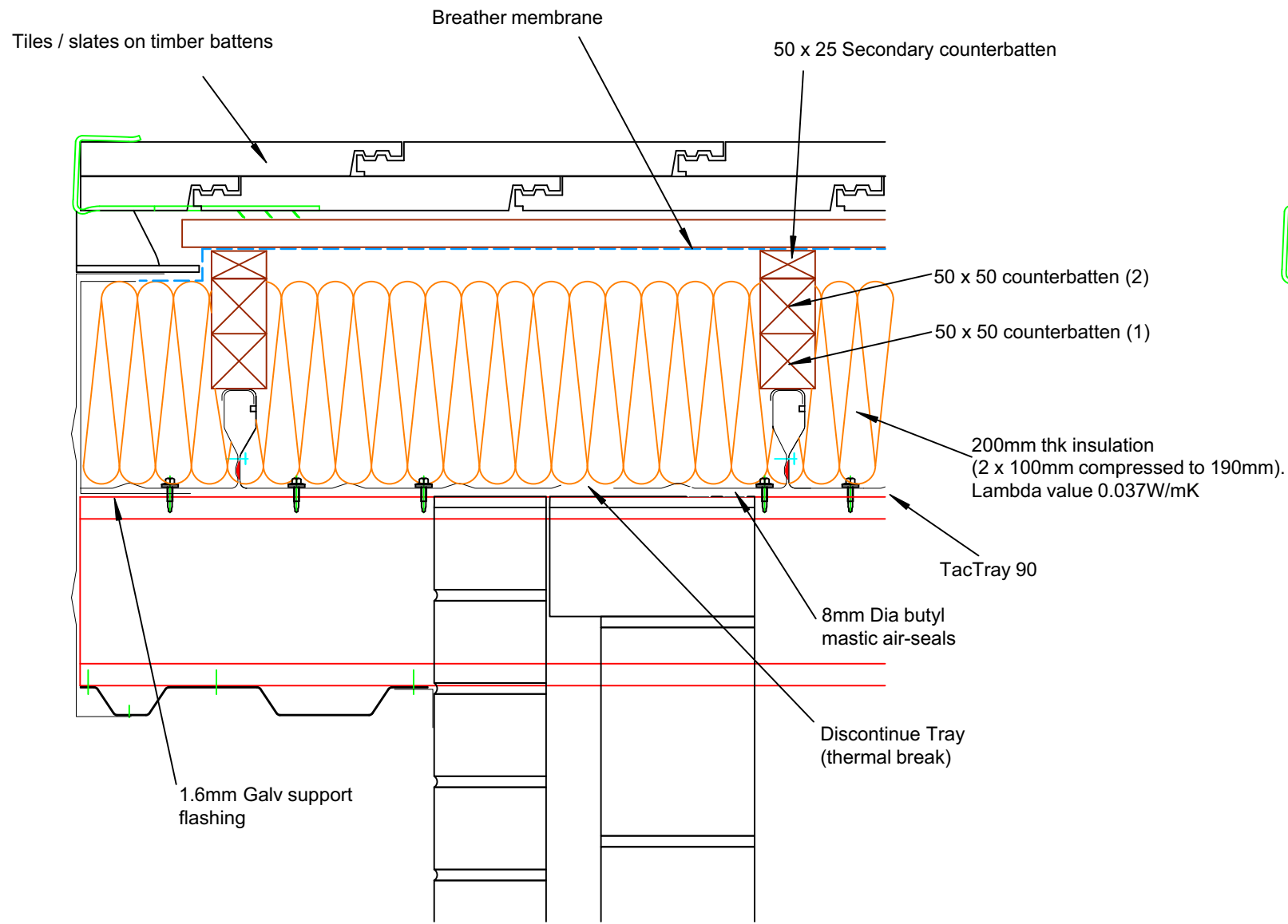
VERGE DETAIL (SOFFITED)
