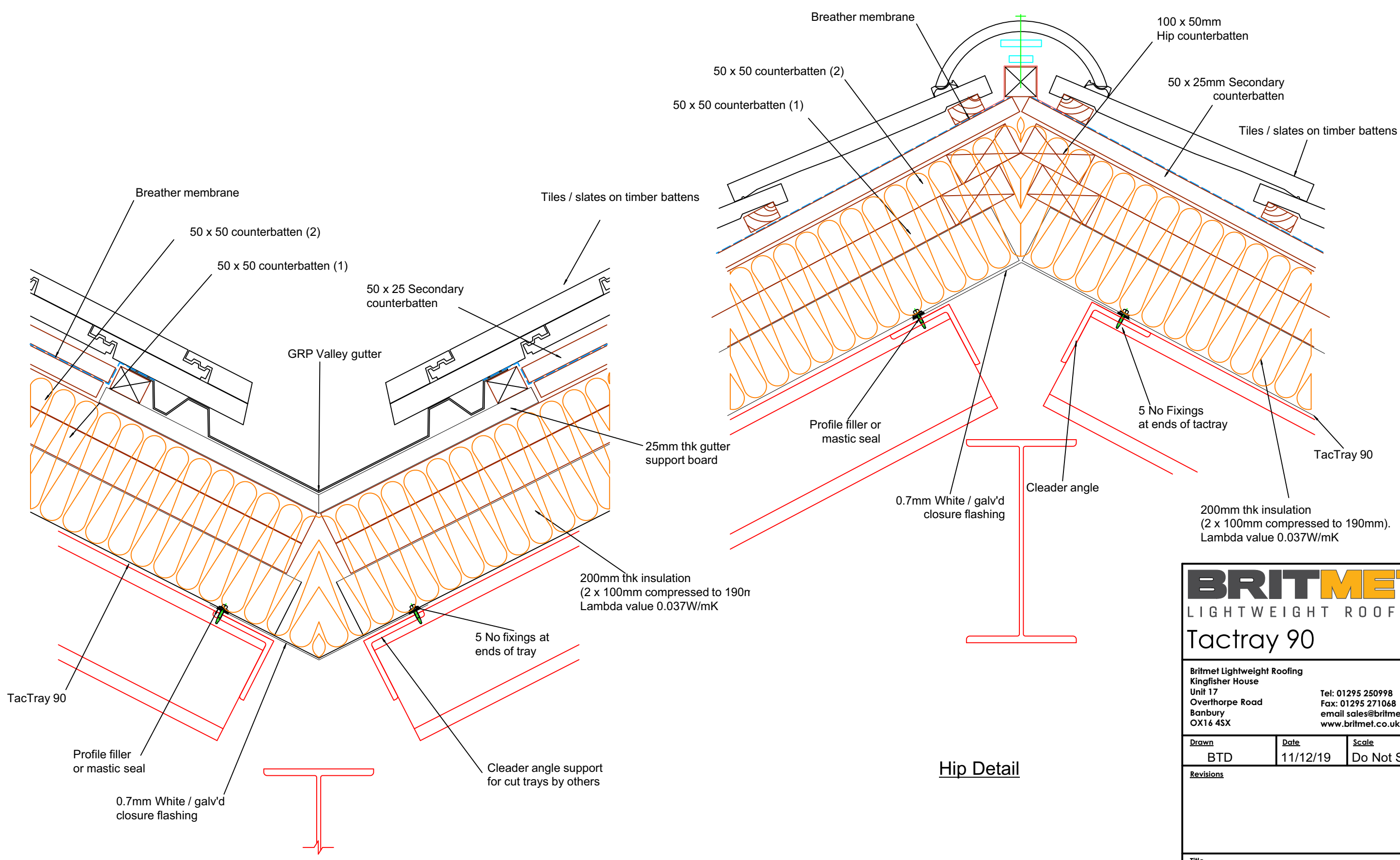
Valley Hip Detail
