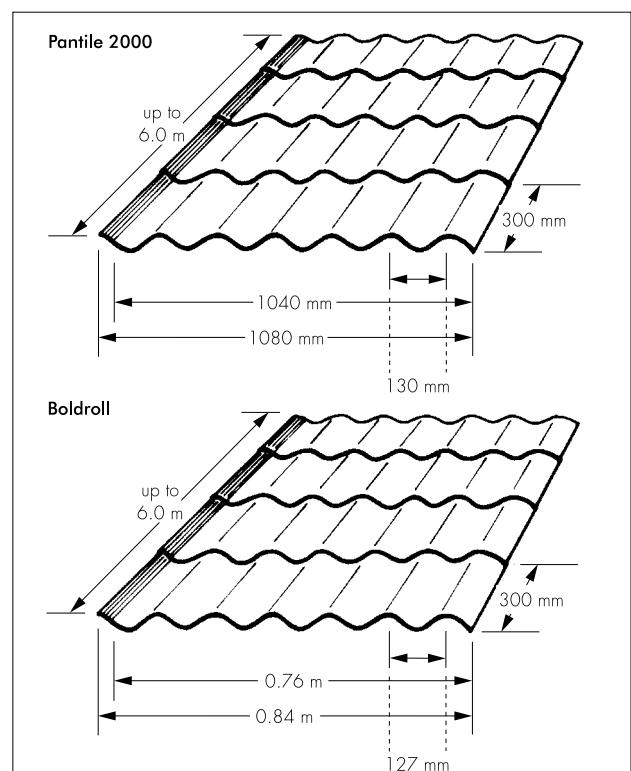
Figure 2 Dimensions
